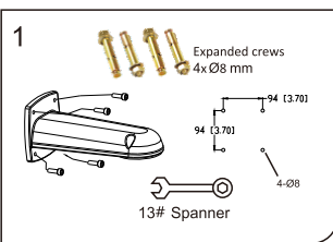
1. Drill 4x holes as above distance. Fix the arm on the wall, and tighten 4x screws as shown in Fig.1.
