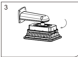
3. Match the circle part with arm, and rotate it to right.
