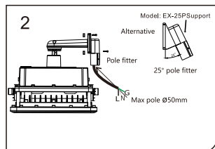
2. Install the pole fitter with arm via 4x M8 screws (The max suitable pole diameter is 50mm). The 25 degree pole fitter could be an alternative.
