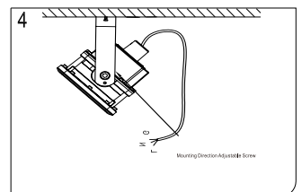
4. Adjust the beam angle from 0 to 180°.
