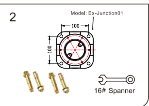
2. Drill 4x φ10mm holes and install the junction box to the wall with M10 expanded screw.
