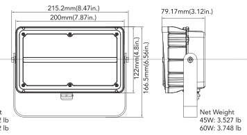
45W&60W(Trunnion Mount)
