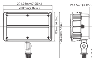
45W&60W(Knuckle Mount)
