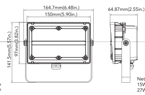
15W&27W(Trunnion Mount)
