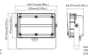
15W&27W(Trunnion Mount)
