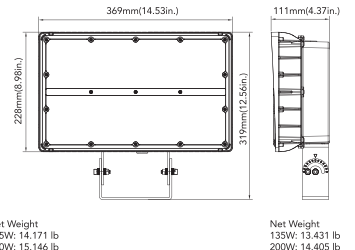
135W&200W(Yoke Mount)
