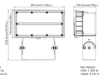
70W&100W(Yoke Mount)
