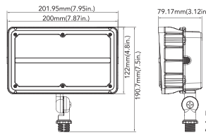
45W&60W(Knuckle Mount)
