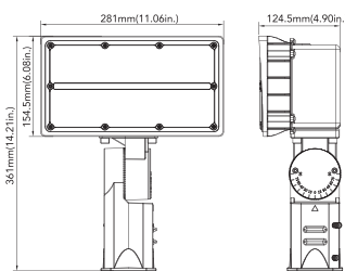
350W(Trunnion Mount)
