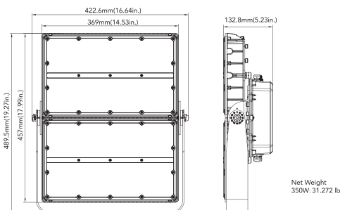
350W(Trunnion Mount)
