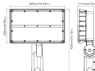
135W&200W(Slipfitter Mount)
