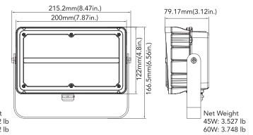
45W&60W(Trunnion Mount)
